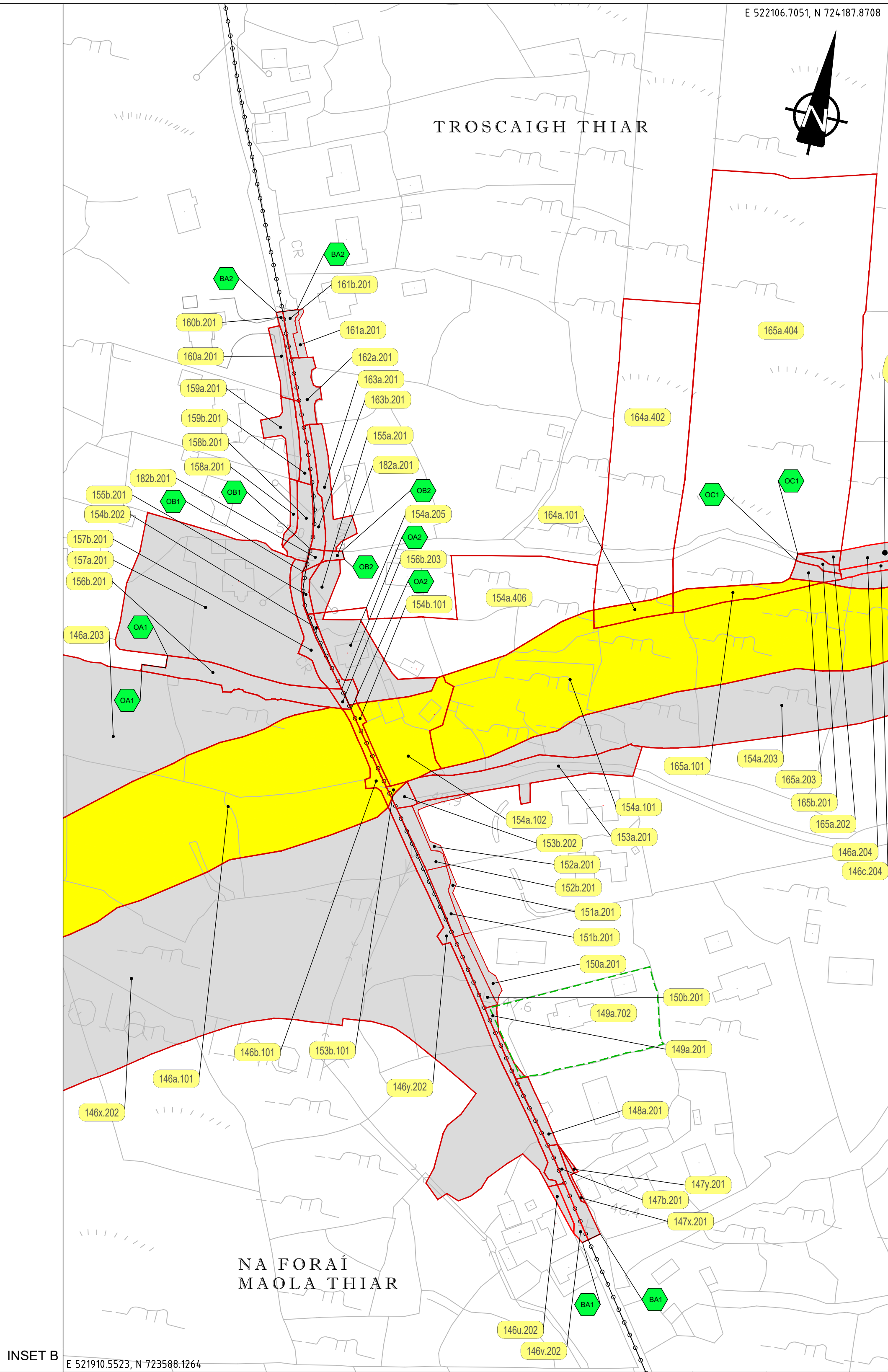
INSET B
